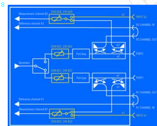
Test set of ZVM and ZVK
